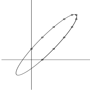
Figure 3: \mu = 1/2 , N = 11 and \theta \approx 0.189 .
