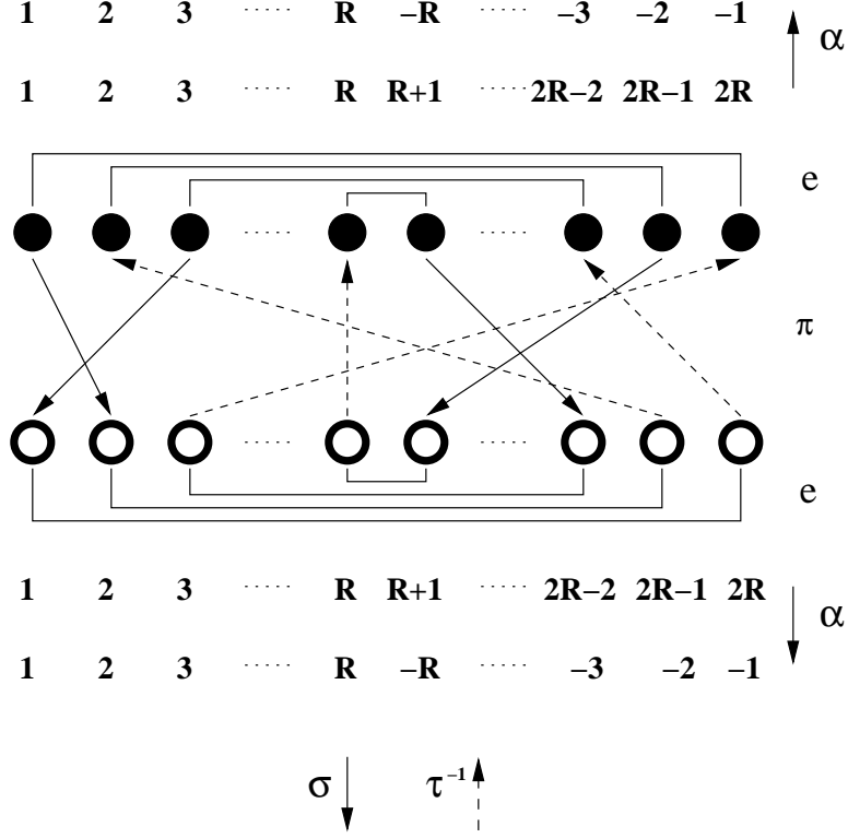
Figure 1: Representation of the bijection. The set of lines, irrespective of their type (solid or dashed) represents \pi \in \mathfrak{S}_{2R} . Solid lines represent \sigma and dashed ones represent \tau . The signs s , resp t , are the signs at the origin, resp. the end, of the solid lines. The arrows, though redundant, are meant to help the reader follow the iterations 1-4 above.
